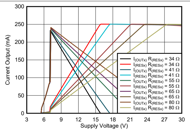
Figure 5-6. Output Current Distribution vs Supply Voltage
