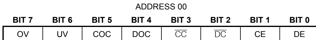
Figure 10. Protection Register Format
