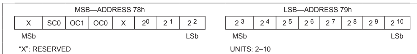
Figure 9. RSGAIN Register
