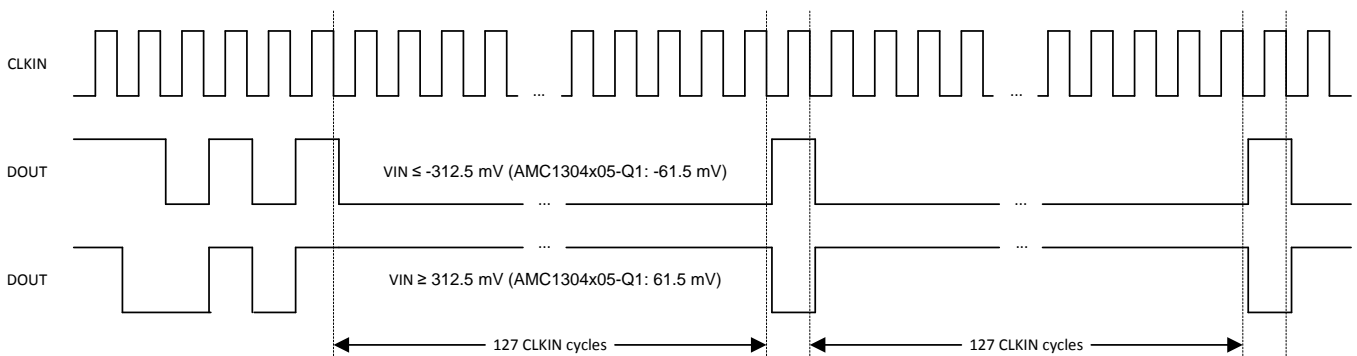
Figure 52. Overage Output of the AMC1304-Q1
