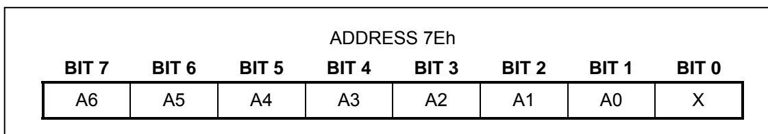
Figure 22. Slave Address Format
