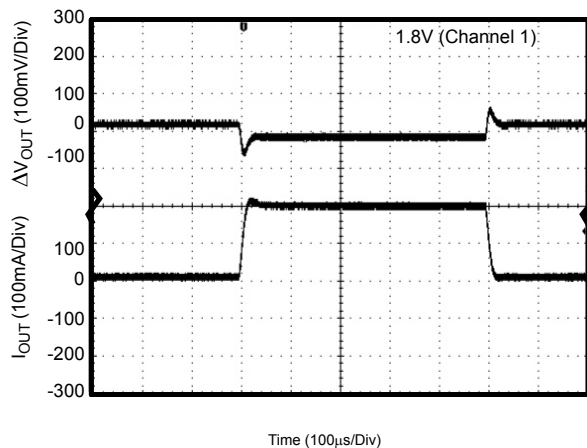
Figure 37. Load Transient
