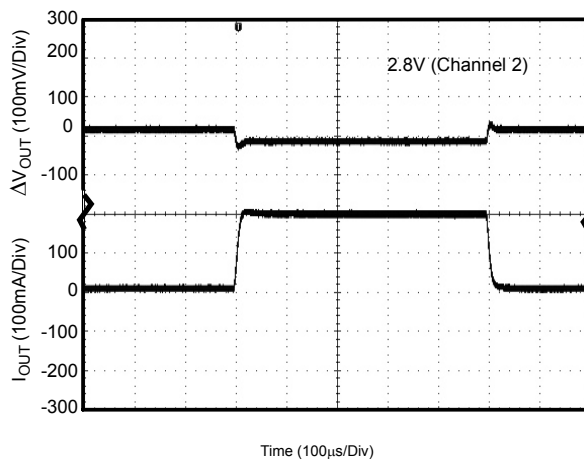
Figure 39. Load Transient
