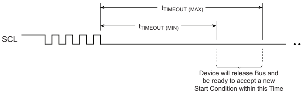
Figure 6-2. SMBus Timeout
