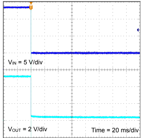
(b. V_{IN} = 13.5\text{ V} \rightarrow 0\text{ V} , C_{OUT} = 2.2\text{ }\mu\text{F} )
