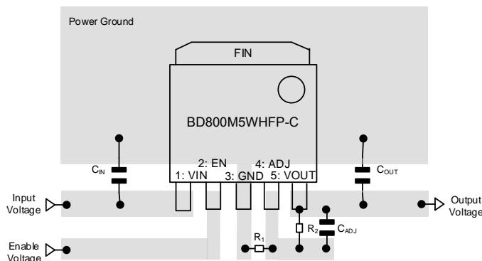
Figure 28. Typical Application and Layout Example
