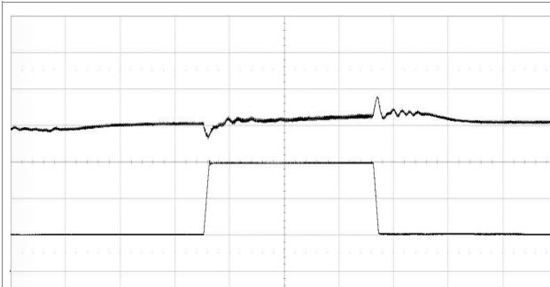
Output Load Transient Response, Opt. PID, Opt.NLR
