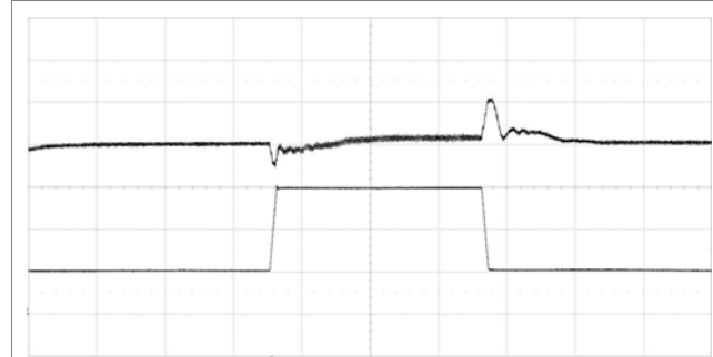
Output Load Transient Response, Opt. PID, default NLR
