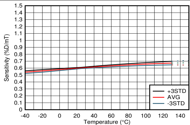
DRV5057A2, V_{CC} = 3.3\text{ V}
