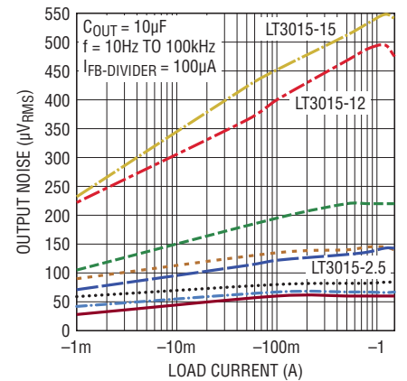
RMS Output Noise vs Load Current
