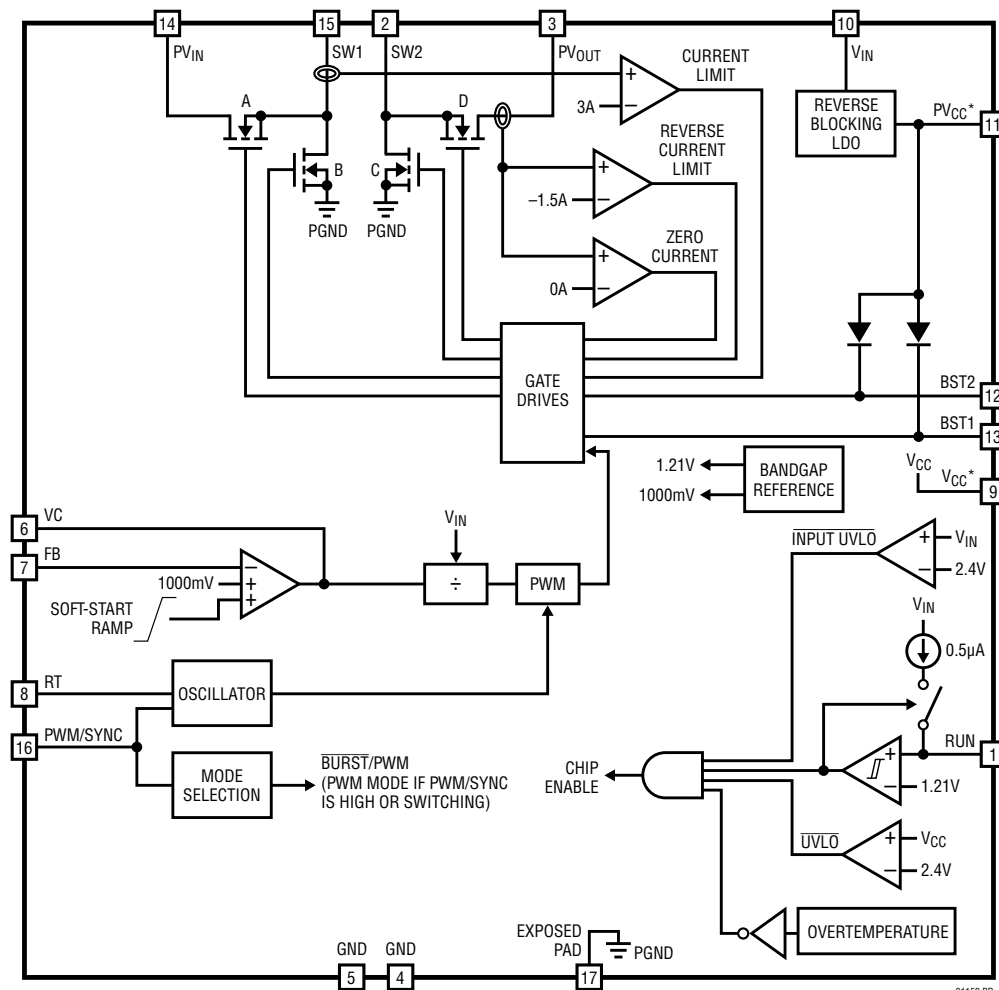
* V_{CC} AND V_{CC} MUST BE CONNECTED TOGETHER IN THE APPLICATION THE EXPOSED PAD IS AN ELECTRICAL CONNECTION AND MUST BE SOLDERED TO THE BOARD AND ELECTRICALLY CONNECTED TO GROUND
