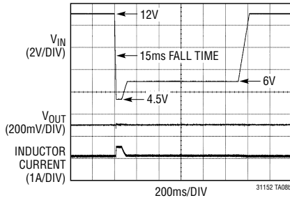
Cold Crank Line Transient with 800mA Load
