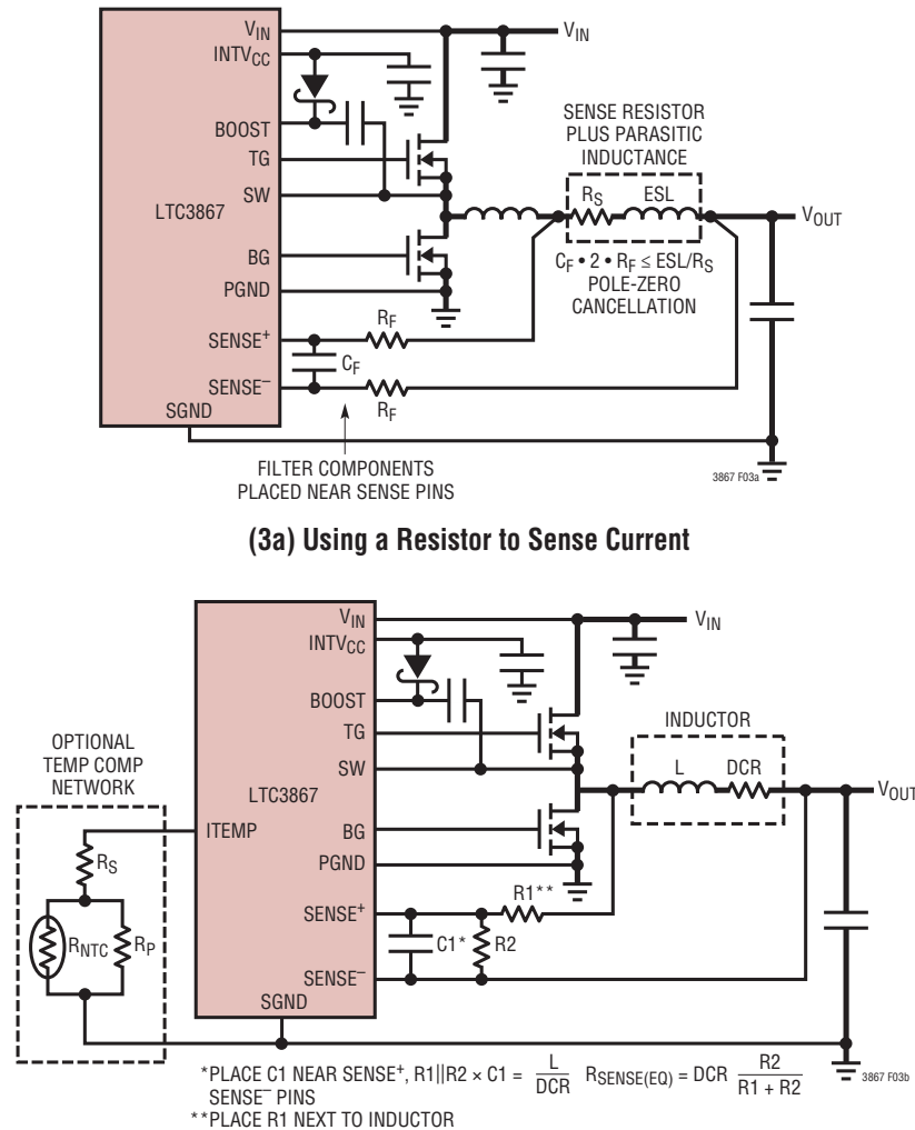
(3b) Using the Inductor DCR to Sense Current
