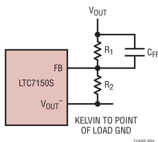
Figure 1. Setting the Output Voltage Differentially
