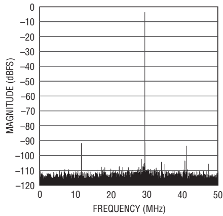
32k-Point FFT, f_{IN} = 70.3\text{MHz} , -1\text{dBFS} , 100Mps
