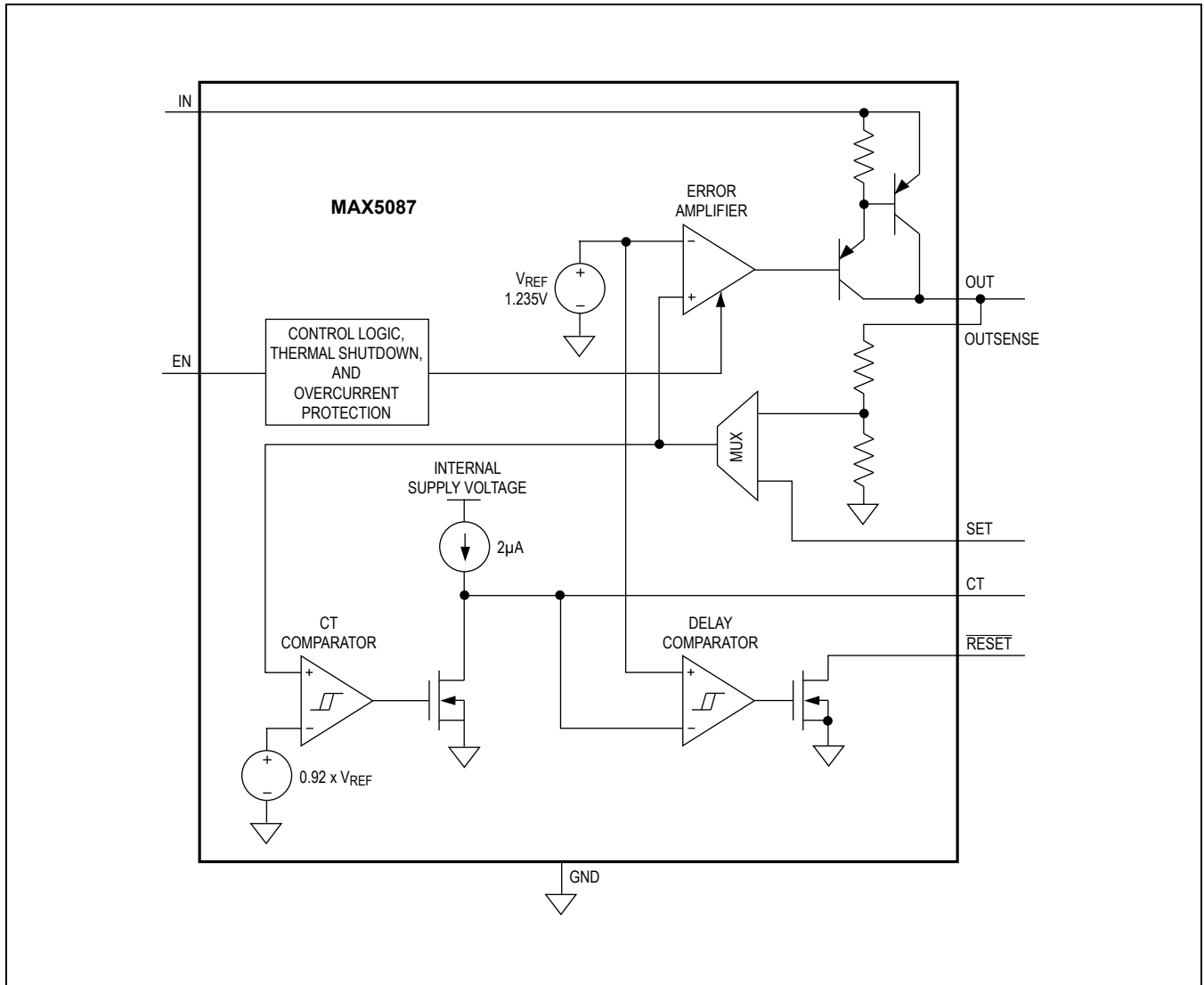
Figure 1. Functional Diagram
