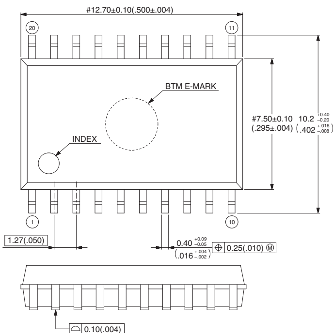
20-pin plastic SOP (FPT-20P-M09)
