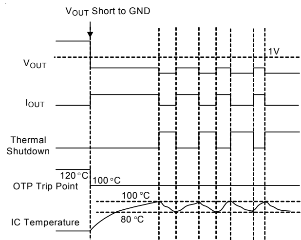
Figure 1. Short Circuit Thermal Folded Back Protection when Output Short Circuit Occurs (Patent)
