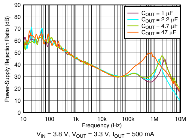
Figure 30. PSRR vs Frequency and C_{OUT}
