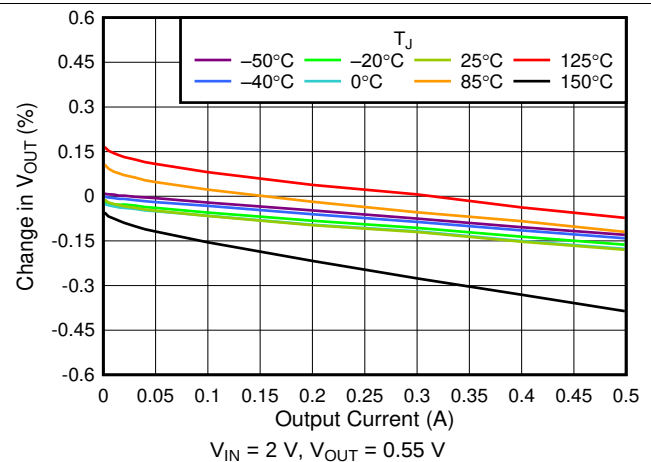
Figure 12. 0.55-V Load Regulation vs I_{OUT}
