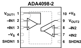
Figure 6. Pin Configuration for ADA4098-2 10-Lead LFCSP
