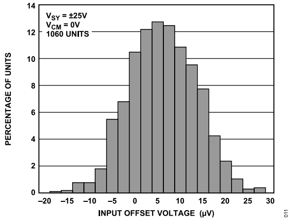
Figure 13. Typical Distribution of Input Offset Voltage with V_{SY} = \pm 25 V
