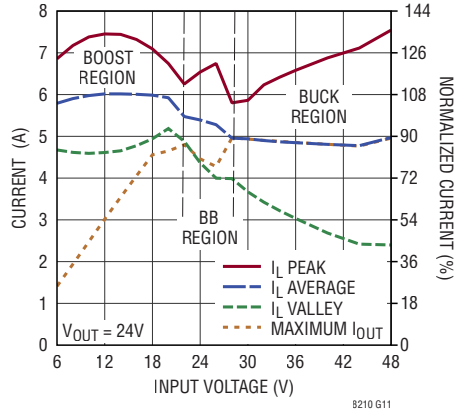
Maximum Inductor Current: f_{sw} = 0.7 \times f_{sw(Optimal)} (Figure 39)
