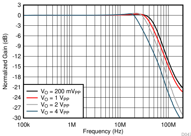
Figure 7. Large-Signal Frequency Response vs Output Voltage
