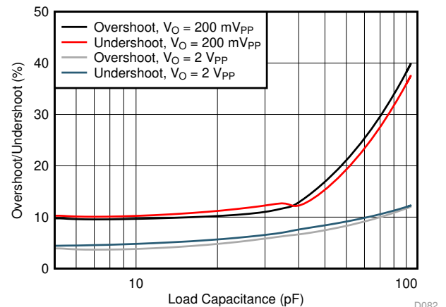
See Figure 64, Gain = 1 V/V, R_F = 0\ \Omega
