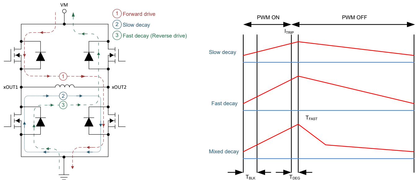
Figure 7-13. Decay Modes
