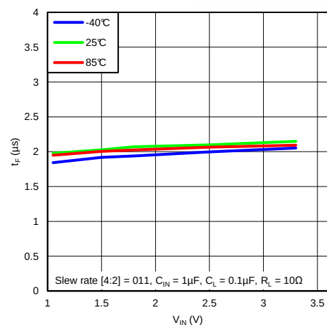
Figure 23. t_{\text{F}} vs. V_{\text{IN}} ( V_{\text{BIAS}} = 7.2\text{V} )
