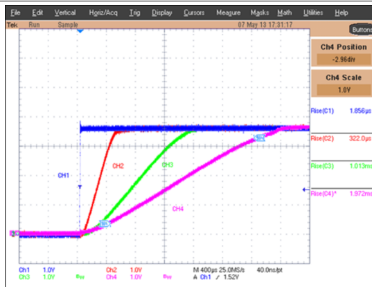
Figure 25. +Power up with different slew rate settings
