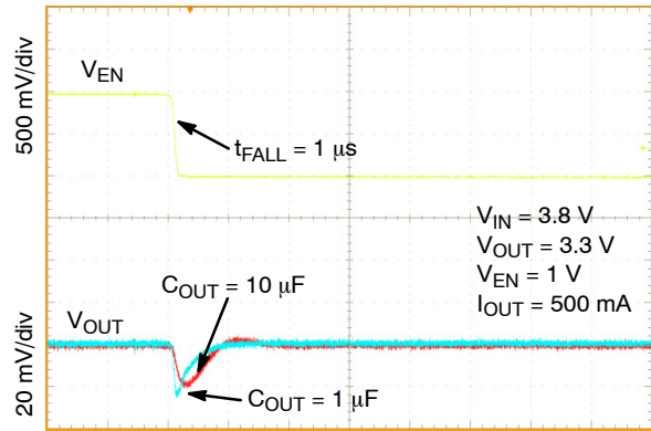
10 \mu s /div Figure 51. Line Transient Response – Falling Edge, V_{OUT} = 3.3 V , I_{OUT} = 500 mA
