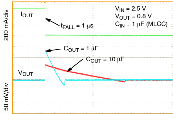
100 \mu s /div Figure 53. Load Transient Response – Falling Edge, V_{OUT} = 0.8 V , I_{OUT} = 1 mA to 500 mA, C_{OUT} = 1 \mu F , 10 \mu F
