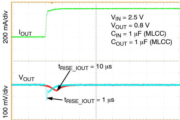
10 \mu s /div Figure 54. Load Transient Response – Rising Edge, V_{OUT} = 0.8 V , I_{OUT} = 1 mA to 500 mA, t_{RISE\_IOUT} = 1 \mu s , 10 \mu s
