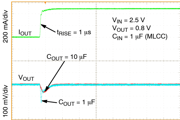
10 \mu s /div Figure 52. Load Transient Response – Rising Edge, V_{OUT} = 0.8 V , I_{OUT} = 1 mA to 500 mA, C_{OUT} = 1 \mu F , 10 \mu F
