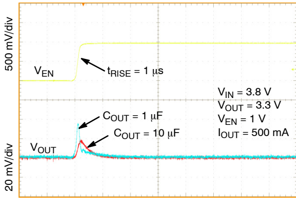
5 \mu s /div Figure 50. Line Transient Response – Rising Edge, V_{OUT} = 3.3 V , I_{OUT} = 500 mA
