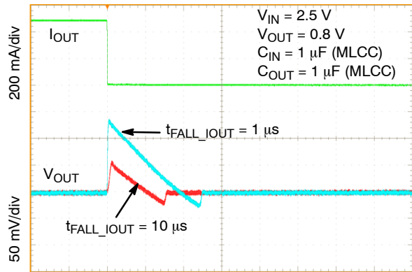
10 \mu s /div Figure 55. Load Transient Response – Falling Edge, V_{OUT} = 0.8 V , I_{OUT} = 1 mA to 500 mA, t_{FALL\_IOUT} = 1 \mu s , 10 \mu s
