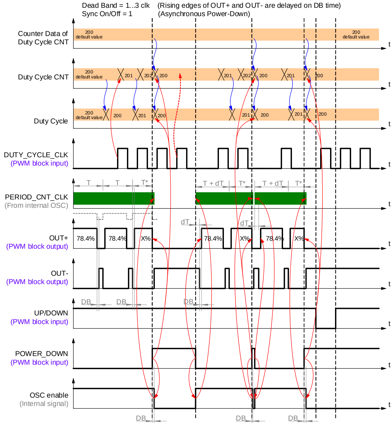
Figure 102: Power-Down with SYNC On/Off = 1 and Dead Band = 1 to 3 CLK
