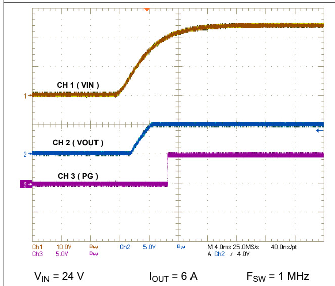
Figure 8-6. Start-up
