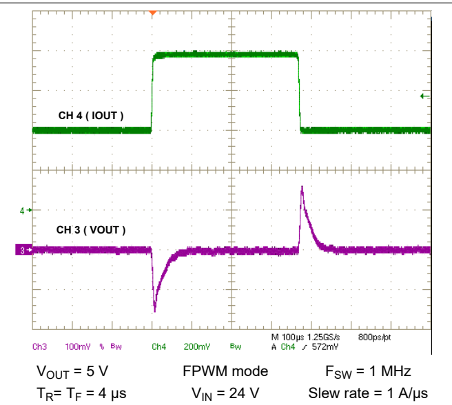
Figure 8-7. Load Transient, 4 A to 8 A, 1 A/μs
