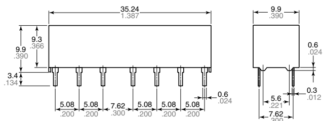
External dimensions
