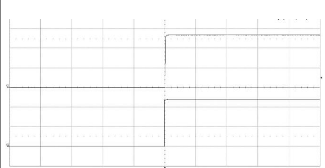
Start-up enabled by connecting V_I at: T_{P1} = +25^\circ\text{C} , V_I = 24\text{ V} , I_O = 0.463\text{ A} resistive load. Top trace: output voltage (20 V/div). Bottom trace: input voltage (10 V/div). Time scale: (200 ms/div.).
