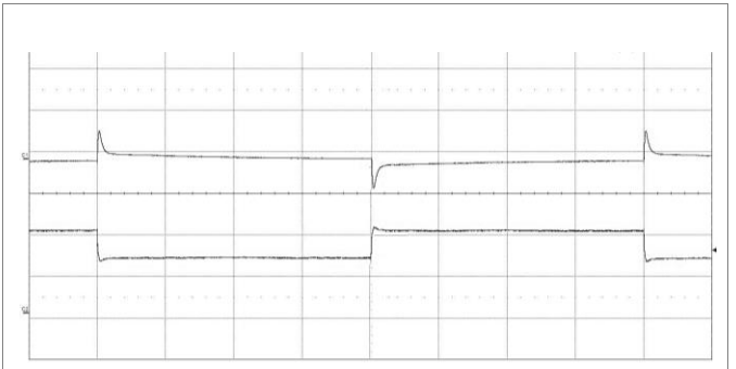
Output voltage response to load current step-change (0.231-0.347-0.231 A) at: T_{P1} = +25^\circ\text{C} , V_I = 24\text{ V} . Top trace: output voltage (500 mV/div.). Bottom trace: load current (200 mA/div.). Time scale: (2 ms/div.).
