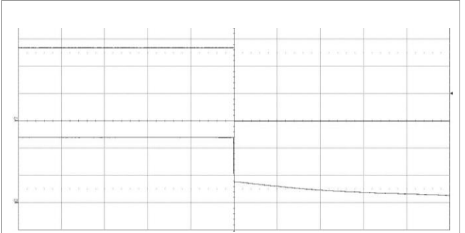
Output disabled by connecting V_I at: T_{P1} = +25^\circ\text{C} , V_I = 24\text{ V} , I_O = 0.463\text{ A} resistive load. Top trace: output voltage (20 V/div.). Bottom trace: input voltage (10 V/div.). Time scale: (200 ms/div.).
