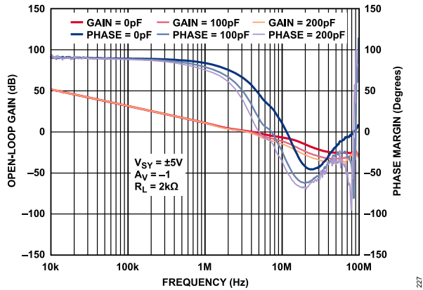
Figure 30. Open-Loop Gain and Phase Margin vs. Frequency, V_{SY} = \pm 5 V
