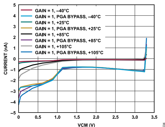
Figure 34. Absolute AINM Current vs. VCM for Various Temperatures (Gain = 1, VDIFF = 0 V)
