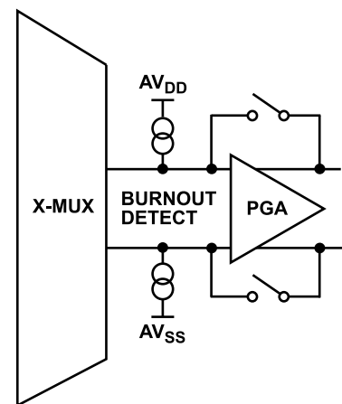
Figure 96. Burnout Currents
