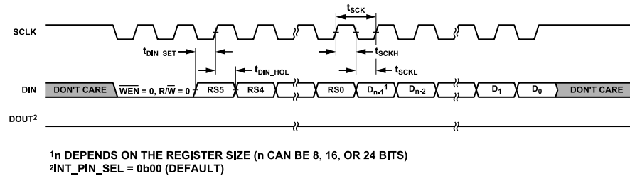
Figure 2. Write Cycle Timing Diagram, 3-Wire Mode ( CSB\_EN Bit Set to 0), \overline{CS} Pin Tied Low
