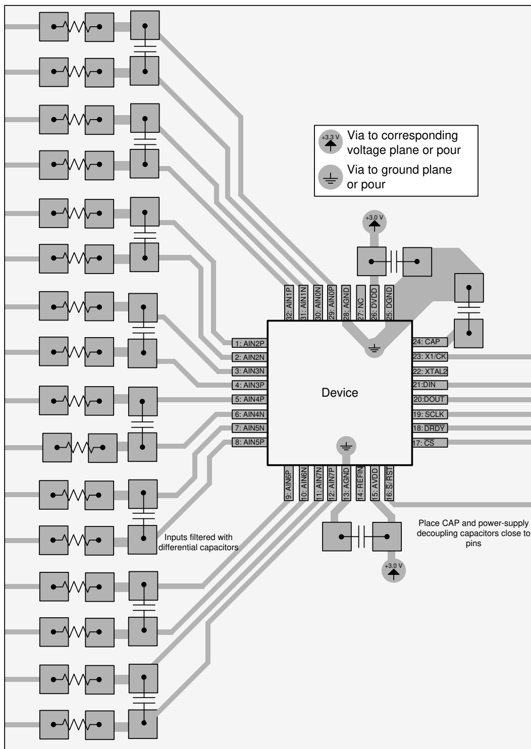
Figure 11-1. Layout Example
