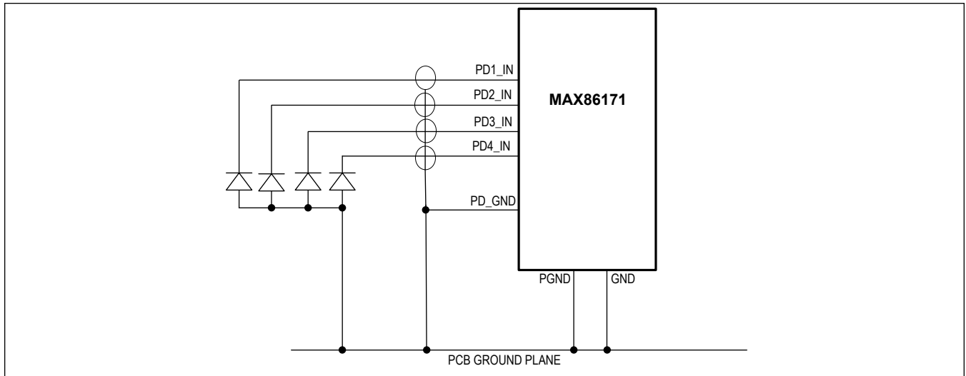
Figure 22. PCB Layout Recommendation
