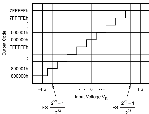
Figure 8-19. Code Transition Diagram
