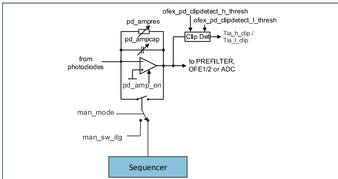
Figure 32: TIA
