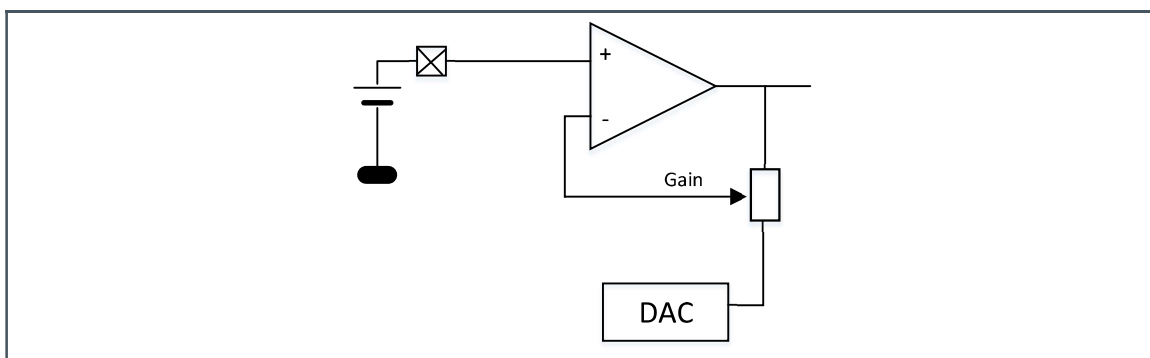
Figure 117: Non Inverting Amplifier High Impedance, GND Referenced
