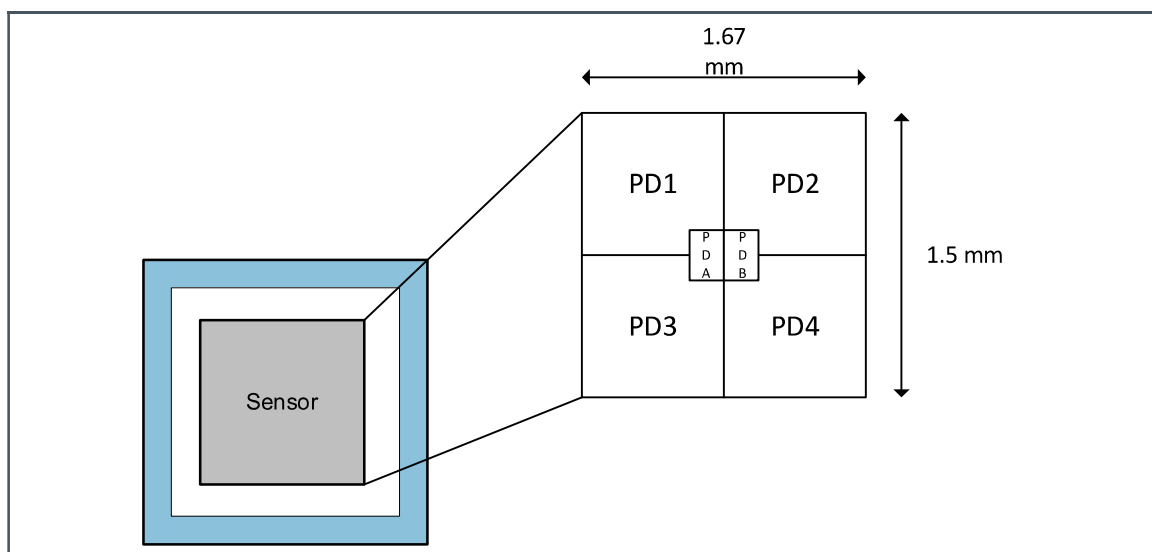
Figure 29: Photodiode Arrangement –Orientation as in Figure 2
