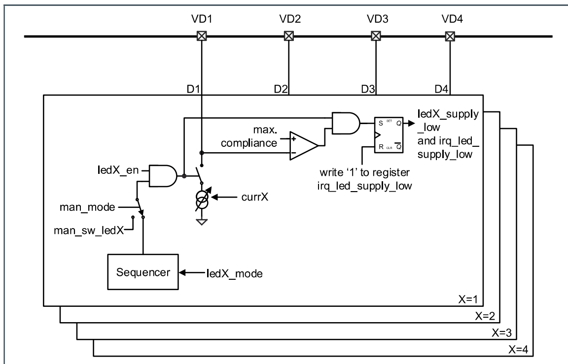
Figure 10: LED Drivers
