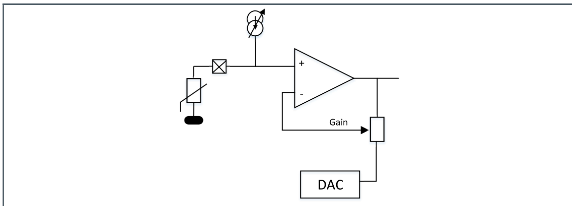
Figure 115: Non Inverting Amplifier with Current Source and Offset (Temperature Sensor)
