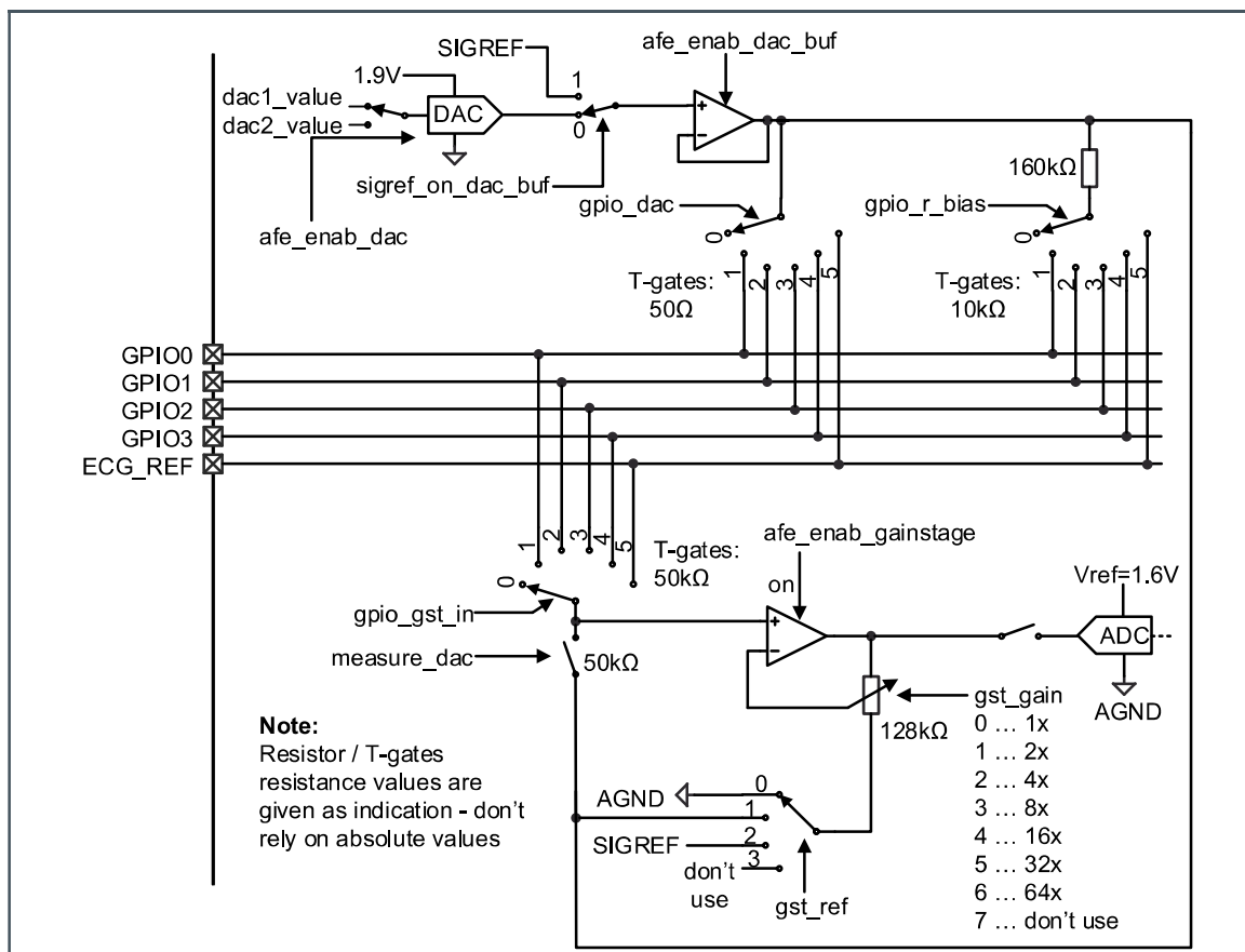
Figure 103: AFE Schematic
