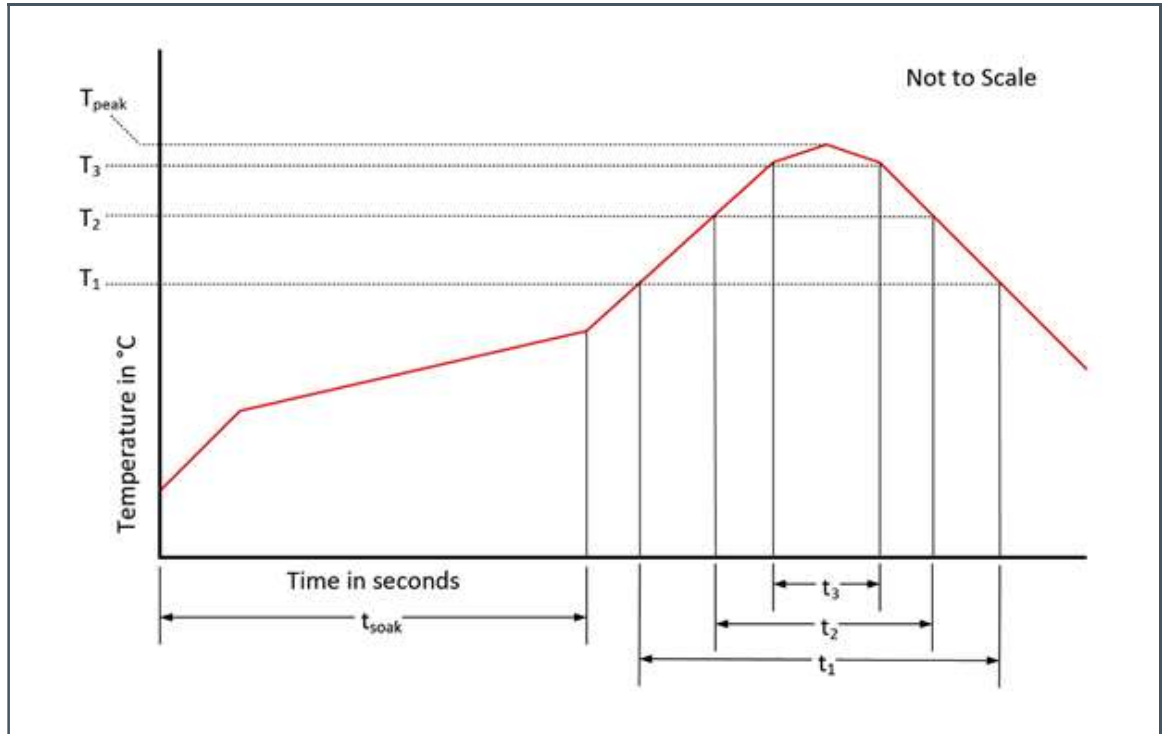
Figure 174: Solder Reflow Profile
