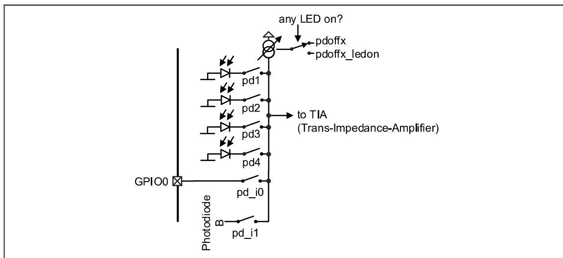
Figure 25: Photodiode Selection
