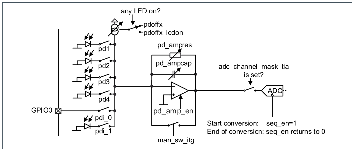
Figure 39: Optical Frontend
