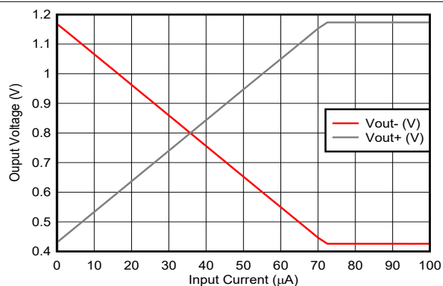
Figure 6-28. Low-Side Swing vs Input Current
