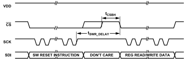
Figure 106. Software Reset Timing Diagram
