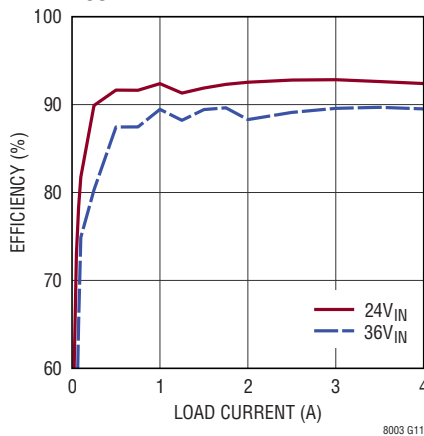
Efficiency vs Load Current, V_{OUT} = -5\text{V} , BIAS Tied to LTM8003 GND
