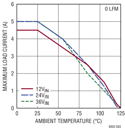
Derating, I-Grade, V_{OUT} = -12\text{V} , BIAS Tied to LTM8003 GND, DC2416A Demo Board
