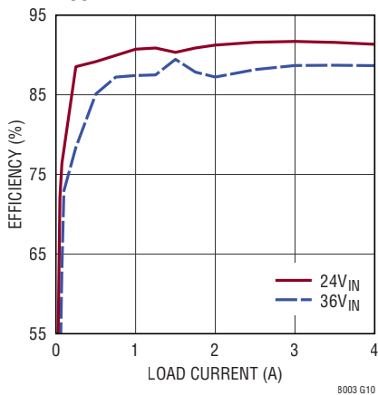
Efficiency vs Load Current, V_{OUT} = -3.3\text{V} , BIAS Tied to LTM8003 GND
