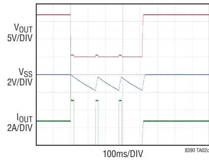
Output Short Protection ( V_{IN} = 12V, I_{OUT} = 3A )
