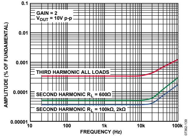
Figure 37. Harmonic Distortion Products vs. Frequency, G = 2
