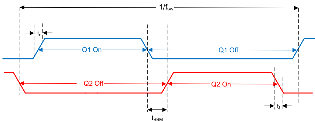
Figure 7-2. Timing Diagram
