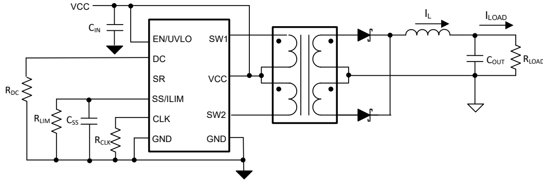
Figure 8-3. Schematic with duty cycle control
