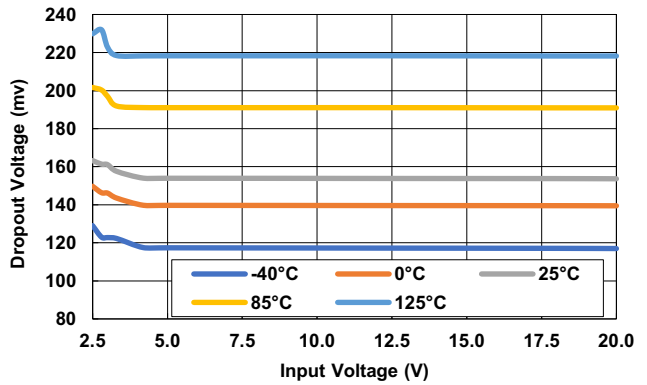
Figure 14. Dropout Voltage vs Input Voltage for Various Junction Temperatures ( I_{OUT} = 300\text{mA} )
