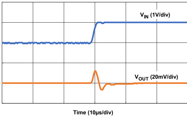
Figure 9. Line Transient Response ( \Delta V_{IN} = 4\text{V to } 5\text{V} in 1\text{V}/\mu\text{s} , V_{OUT} = V_{ADJ} , I_{OUT} = 500\text{mA} , C_{FF} = \text{None} , C_{OUT} = 2.2\mu\text{F} )
