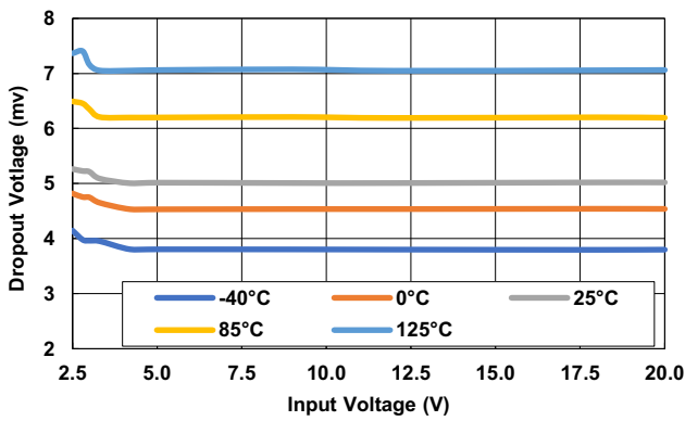
Figure 11. Dropout Voltage vs Input Voltage for Various Junction Temperatures ( I_{OUT} = 10\text{mA} )
