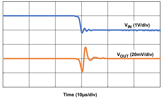
Figure 10. Line Transient Response ( \Delta V_{IN} = 5\text{V to } 4\text{V} in 1\text{V}/\mu\text{s} , V_{OUT} = V_{ADJ} , I_{OUT} = 500\text{mA} , C_{FF} = \text{None} , C_{OUT} = 2.2\mu\text{F} )
