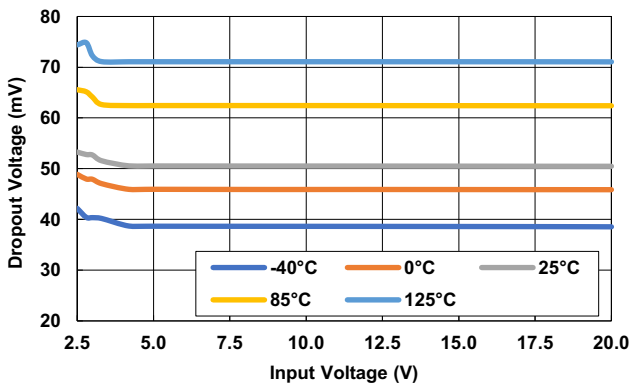
Figure 13. Dropout Voltage vs Input Voltage for Various Junction Temperatures ( I_{OUT} = 100\text{mA} )
