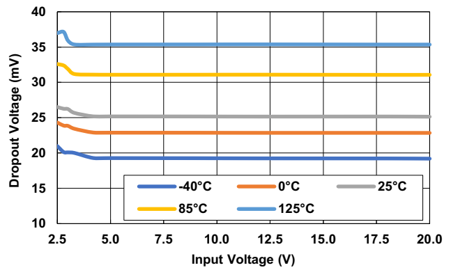
Figure 12. Dropout Voltage vs Input Voltage for Various Junction Temperatures ( I_{OUT} = 50\text{mA} )
