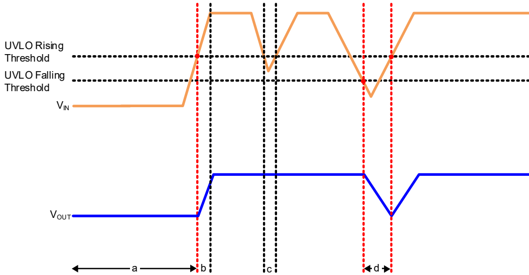
Figure 75. UVLO Operation
