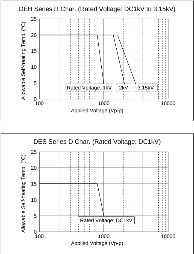
<Fig. 1> Relationship Between Applied Voltage and Self-heating Temperature (Allowable Self-heating Temp. at 25°C Ambient Temp.)
