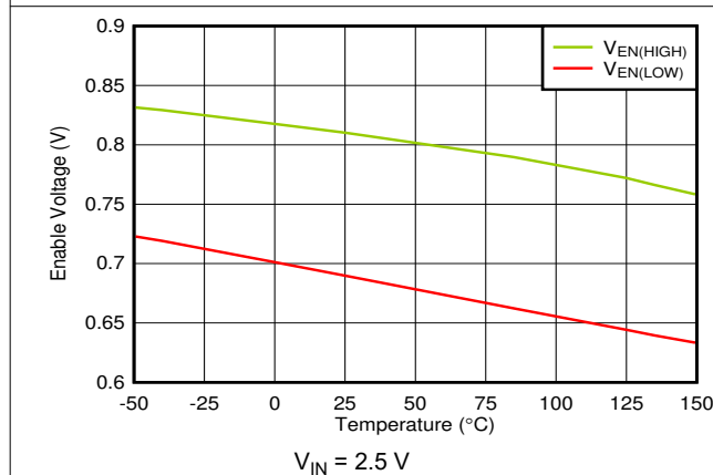
Figure 7-23. V_{EN} Thresholds vs Temperature
