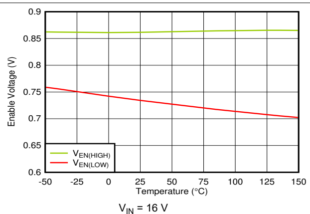
Figure 7-24. V_{EN} Thresholds vs Temperature
