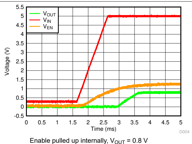
Figure 7-22. Startup With V_{EN} Floating
