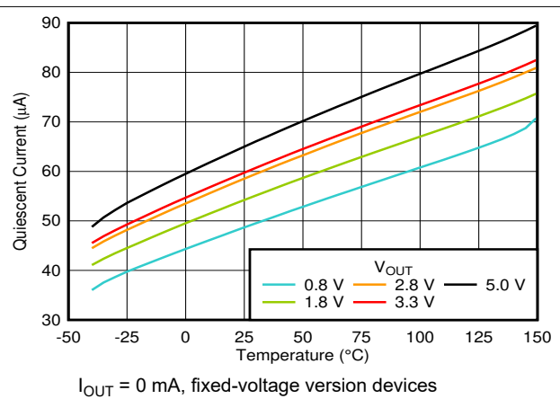
Figure 7-6. I_Q vs Temperature
