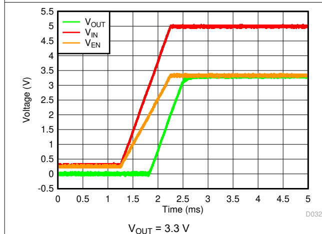
Figure 7-21. Startup With Separate V_{EN} and V_{IN}
