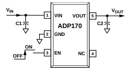
Figure 1. ADP170 with Fixed Output Voltage, 1.8 V
