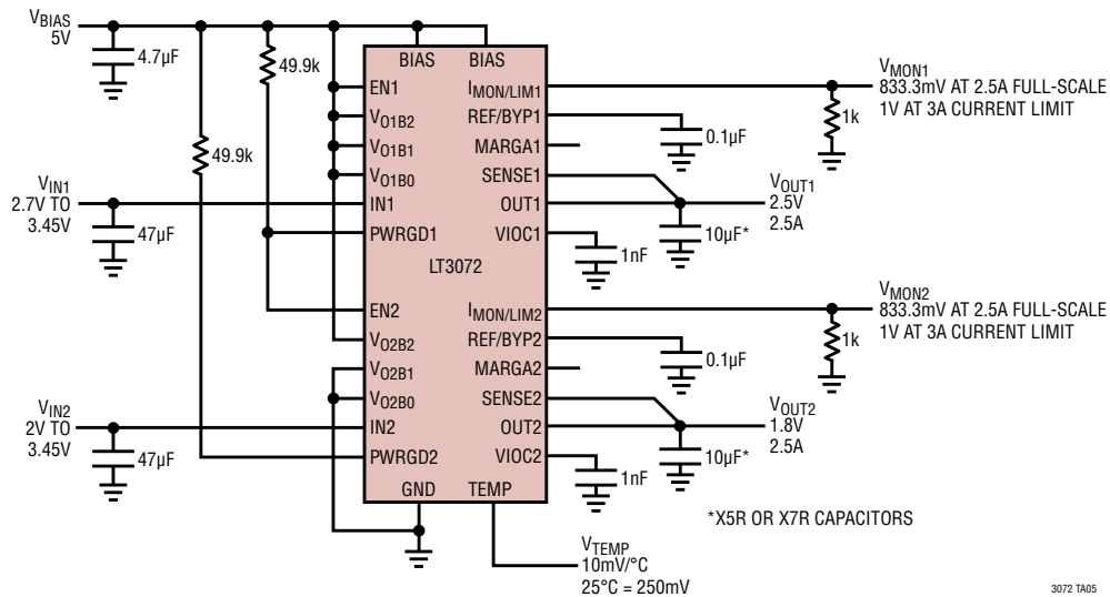
BIAS/2.5V/1.8V Supply Sequencing
