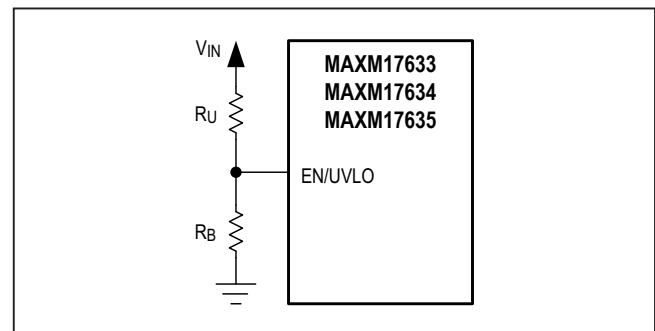
Figure 1. Setting the EN/UVLO Network
