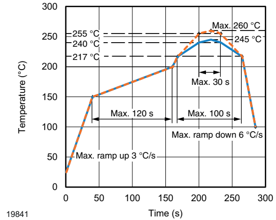
Fig. 16 - Lead (Pb)-free Reflow Solder Profile According to J-STD-020
