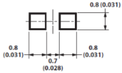
Recommended Solder Pad
