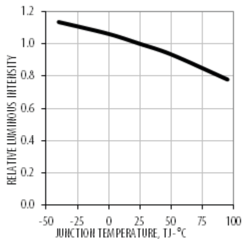
Figure 6 Relative Intensity vs. Temperature
