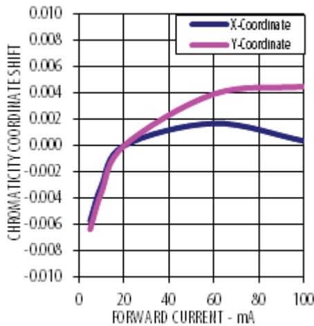
Figure 5 Chromaticity Shift vs. Forward Current
