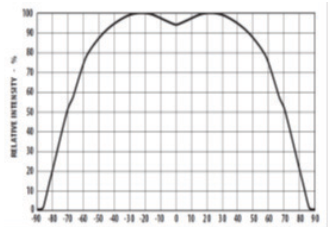
Figure 4 Radiation Pattern
