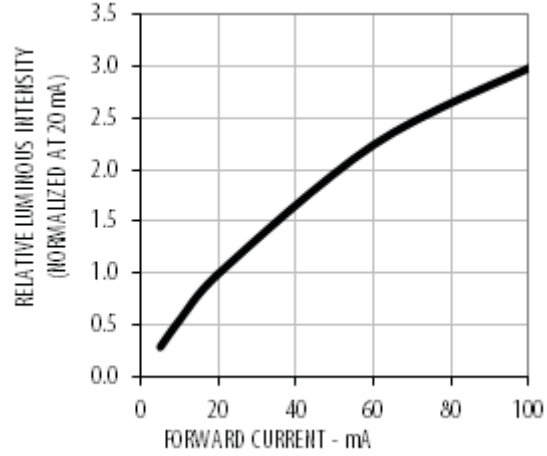
Figure 2 Luminous Intensity vs. Forward Current
