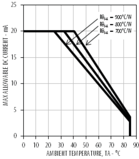
Figure 7 Derating Curve
