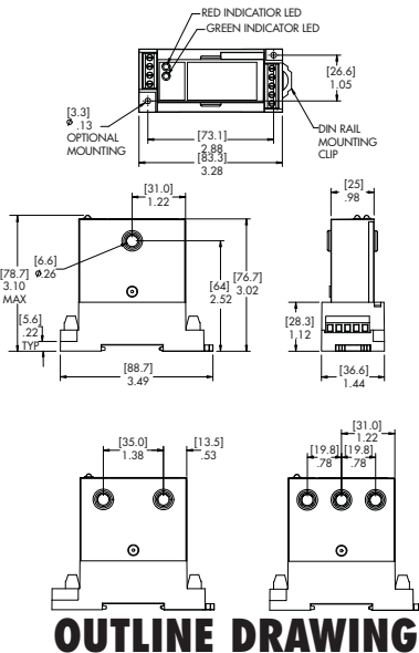
CRD4150 Dual Element, 3-Wire
